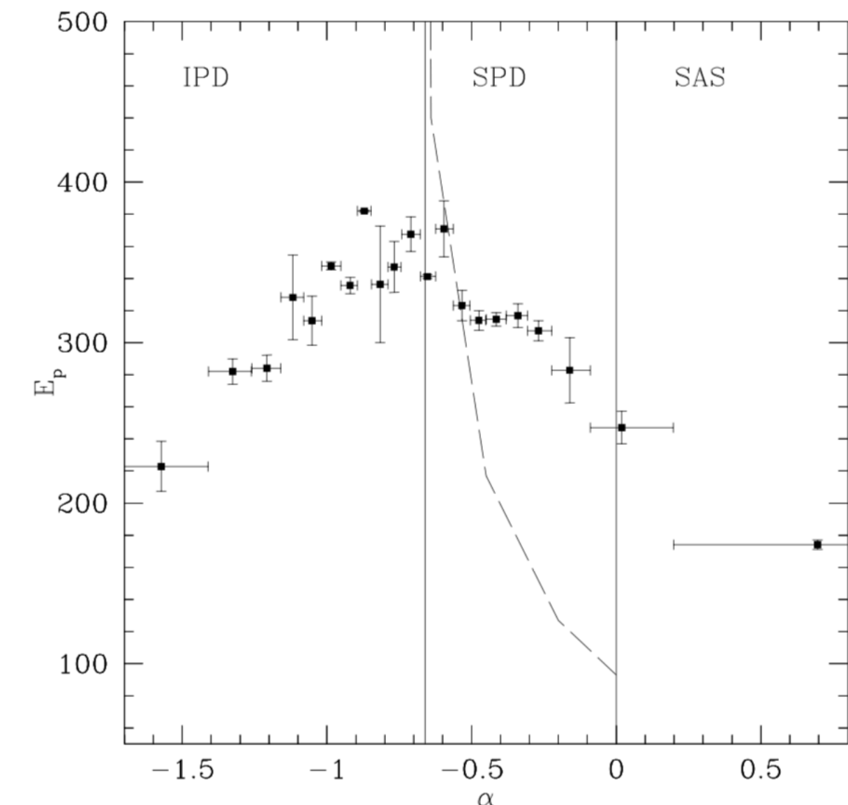
The observed E_p - \alpha correlation in an example BATSE burst. The vertical lines separate different physical regimes. The dashed line shows the expected E_p - \alpha trend for decreasing mean electron synchrotron pitch angle.
