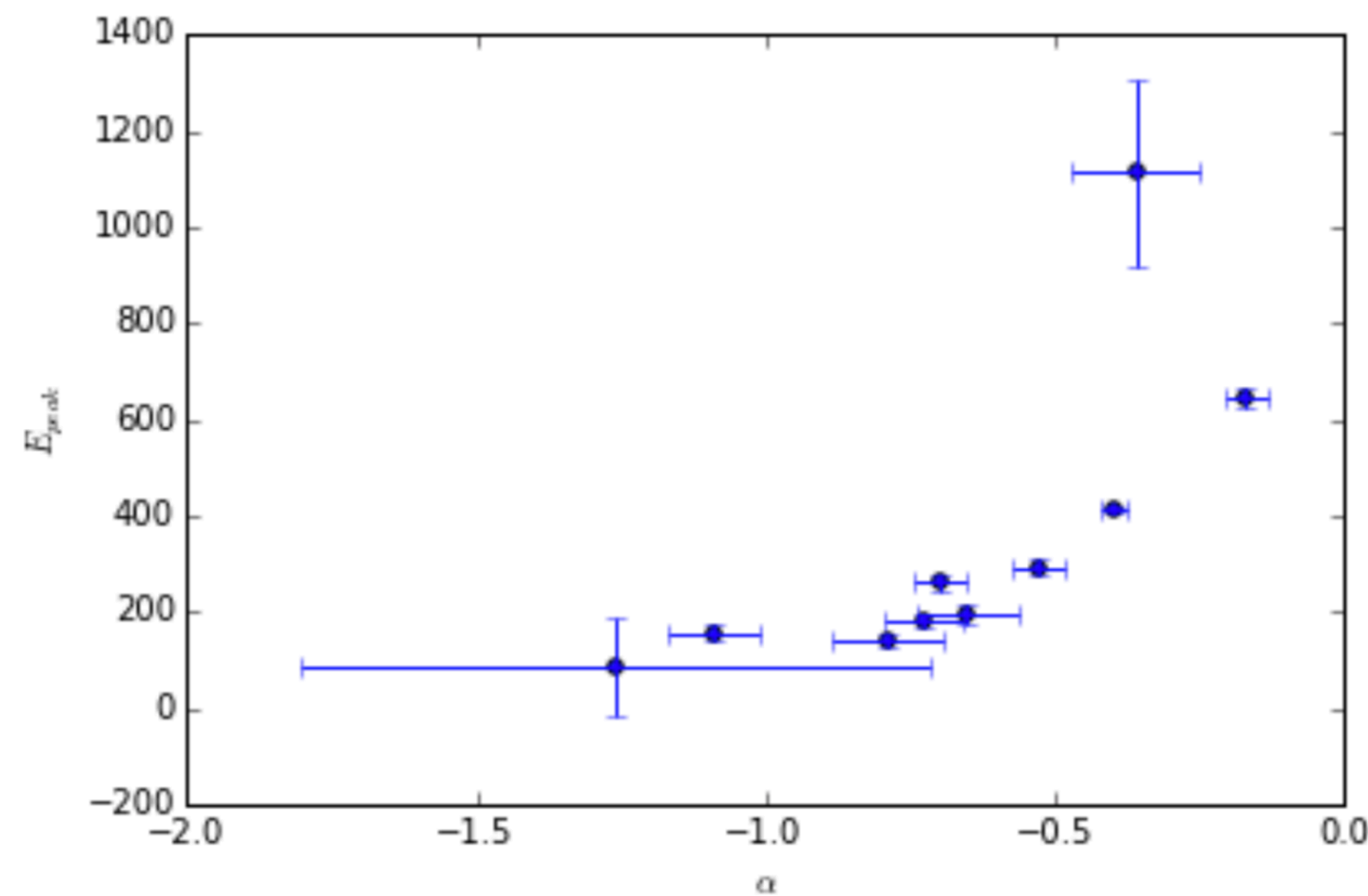
The fit E_p - \alpha correlation for an example GBM burst.
