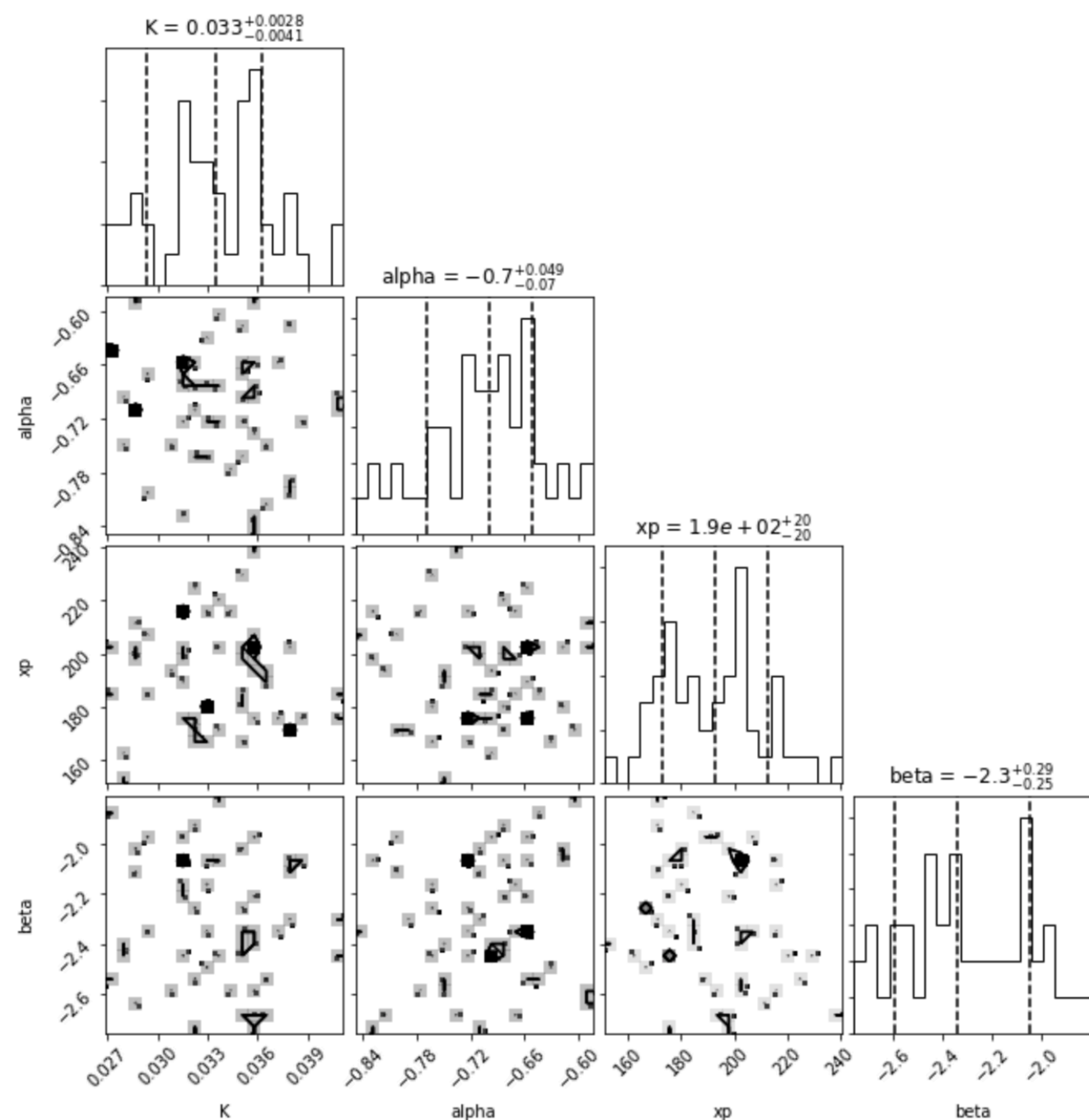
Bayesian “corner plot” example obtained using 3ML.
