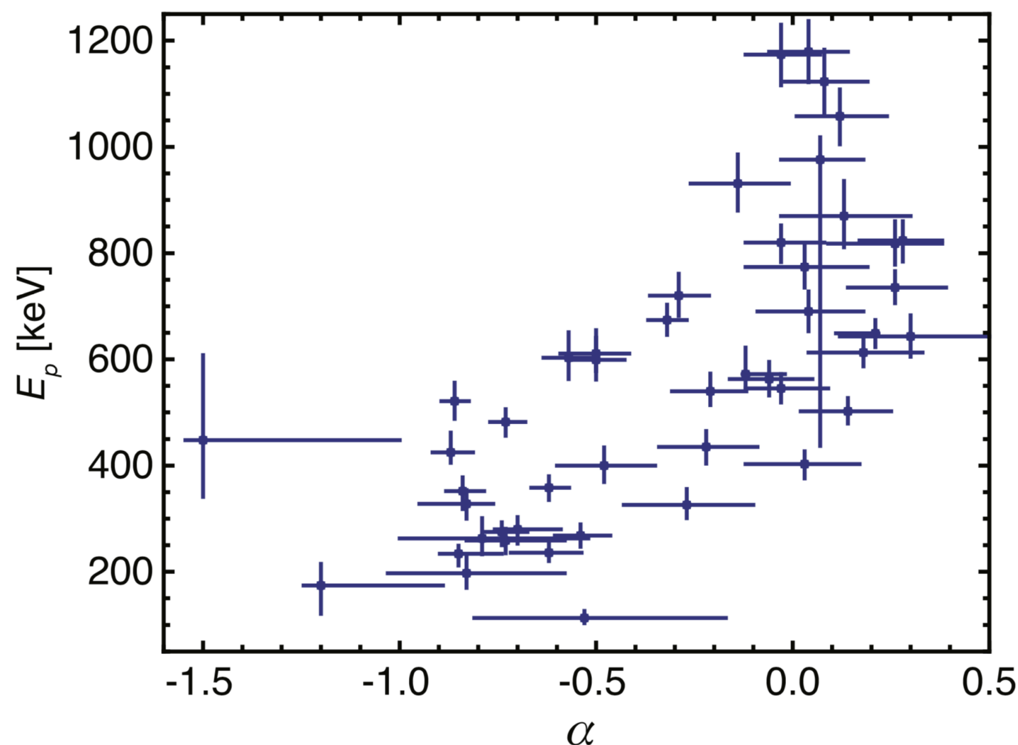
The observed E_p - \alpha correlation in the GBM burst GRB090902B. The correlation could be explained by a sub-photospheric dissipative thermal emission model.
