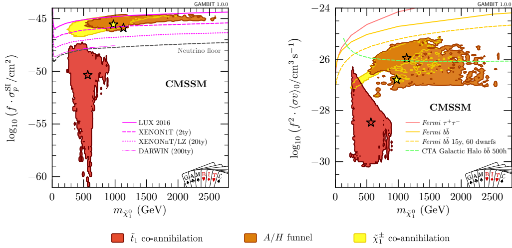
Figure 3: 95% confidence regions of the Constrained Minimal Supersymmetric SM (CMSSM) [28], in terms of the DM mass m_{\tilde{\chi}_1^0} and its rescaled spin-independent scattering cross-section with protons ( left ) or self-annihilation cross-section ( right ). Shading indicates processes able to deplete the relic density. Stars are the best fits in each region. Direct and indirect signals have been rescaled to self-consistently account for the thermal DM relic abundance, but for display, the cross-sections have been rescaled in compensation, to allow comparison with official 90% confidence limits from LUX [29], 95% limits from Fermi -LAT searches towards dwarf galaxies [24], and projections from XENON [30], DARWIN [31], Fermi [32] and CTA [33]. The dashed grey line indicates the expected ‘neutrino floor’ for direct detection [34].
