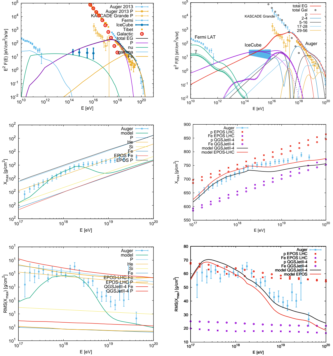
Figure 1: Predictions for the diffuse flux (top) of five elemental groups together with the proton (orange errorbars) and total flux from KASCADE, KASCADE-Grande (light-blue errorbars) [8] and Auger (dark-blue errorbars) [7], the EGRB from Fermi-LAT (light-blue errorbars) [2], and the high-energy neutrino flux from IceCube (light-blue shaded area) [3]. Crosses and dotted lines denote neutrinos and photons from A\gamma and Ap interaction, respectively. The middle and lower panels compare predictions for X_{\max} and \text{RMS}(X_{\max}) using the EPOS-LHC [19] and QGSJET-II-04 [15] models to data from Auger [7]. Left panels for only hadronic interactions with \alpha = 1.8 , E_{\max} = 3 \times 10^{18} eV and BL Lac evolution. Right panels for both A\gamma and Ap interactions with \alpha = 1.5 , E_{\max} = 6 \times 10^{18} eV, \tau^{p\gamma} = 0.29 and AGN evolution. The hadronic interaction depth is normalised as \tau_0^{pp} = 0.035 .
