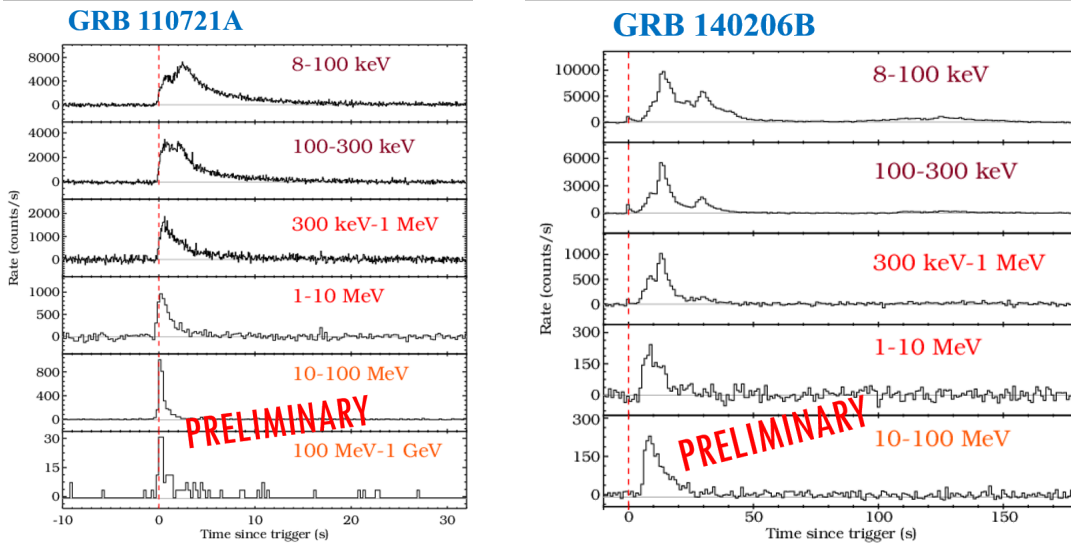
Figure 1: Lightcurves of two LAT-detected long GRBs, GRB 110721a (left plot) and GRB 140206B (right plot) as seen at different energies.
