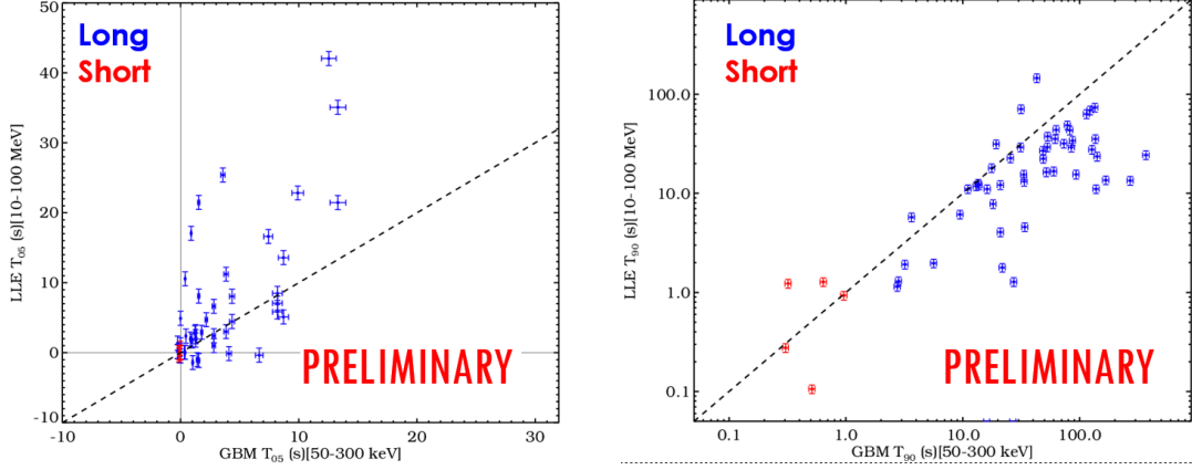
Figure 2: Distribution of T_{05} and T_{90} measured from LLE data in the 10–100 MeV energy range versus the same quantities measured from GBM NaI data in the 50–300 keV energy range.
