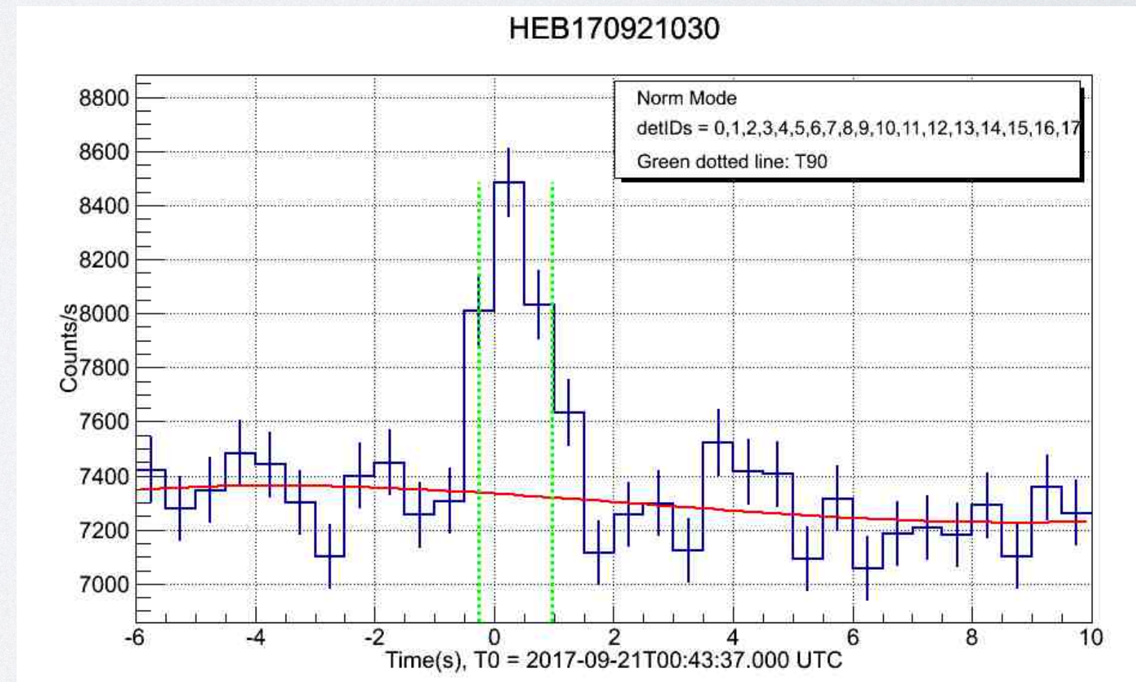
Insight-HXMT lightcurve
