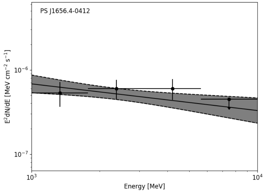
Fig 3 NGC 6254 Power law with prefactor (6.7 \pm 1.4) \times 10^{-13} , index -2.3 \pm 0.18 , scale 1000.
